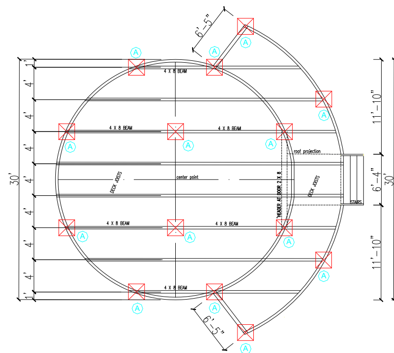
2 -SCHEMATIC DECK FRAMING
